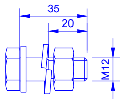
14 M12x35x20+P(1)+AP(1)+AM(1) (Esc 1/2)
