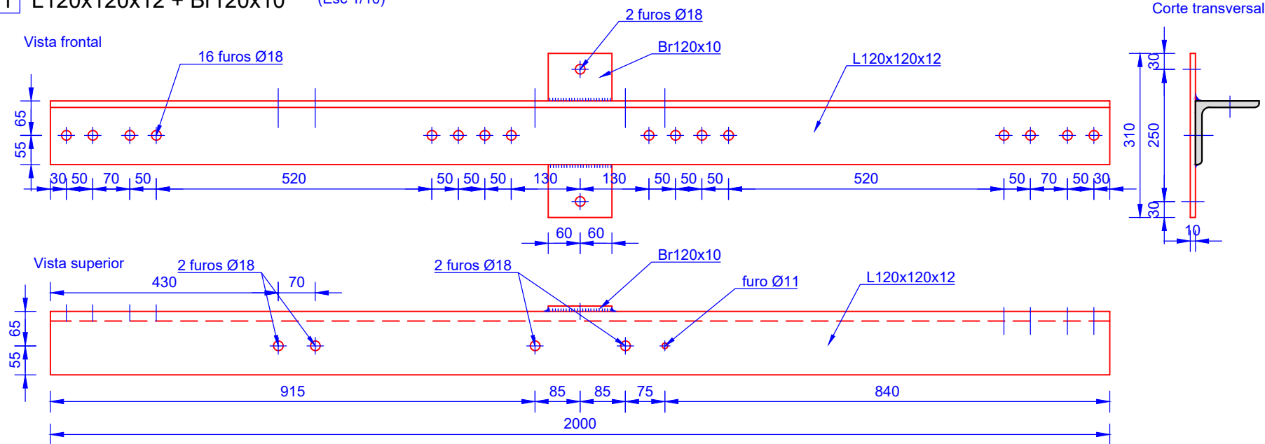
1 L120x120x12 + Br120x10 (Esc 1/10)
