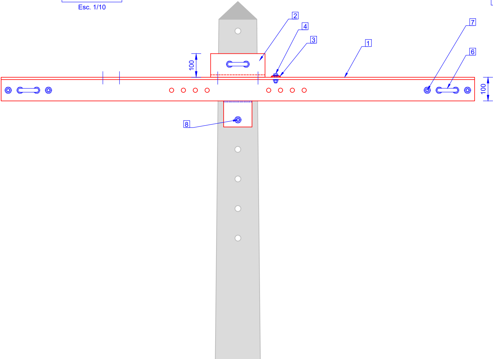
Vista frontal
