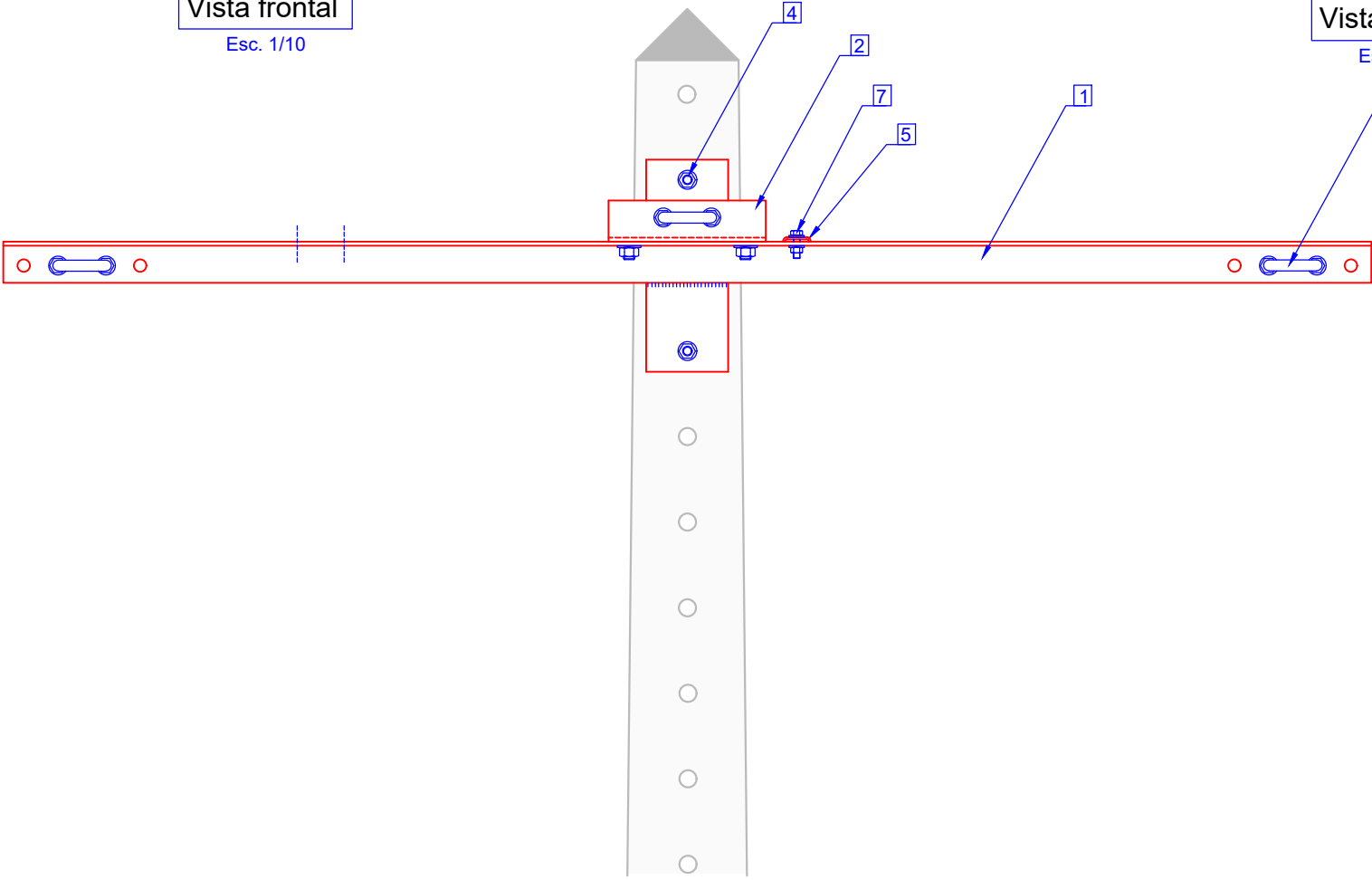
Vista frontal
