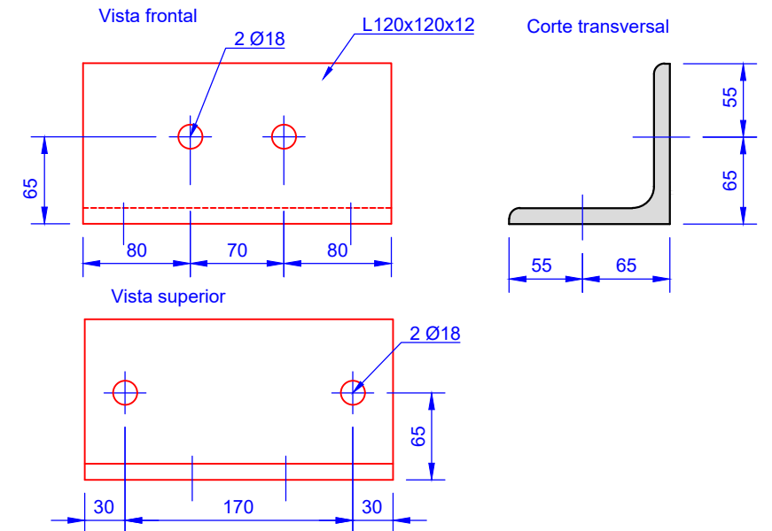
2 L120x120x12 (Esc 1/5)
