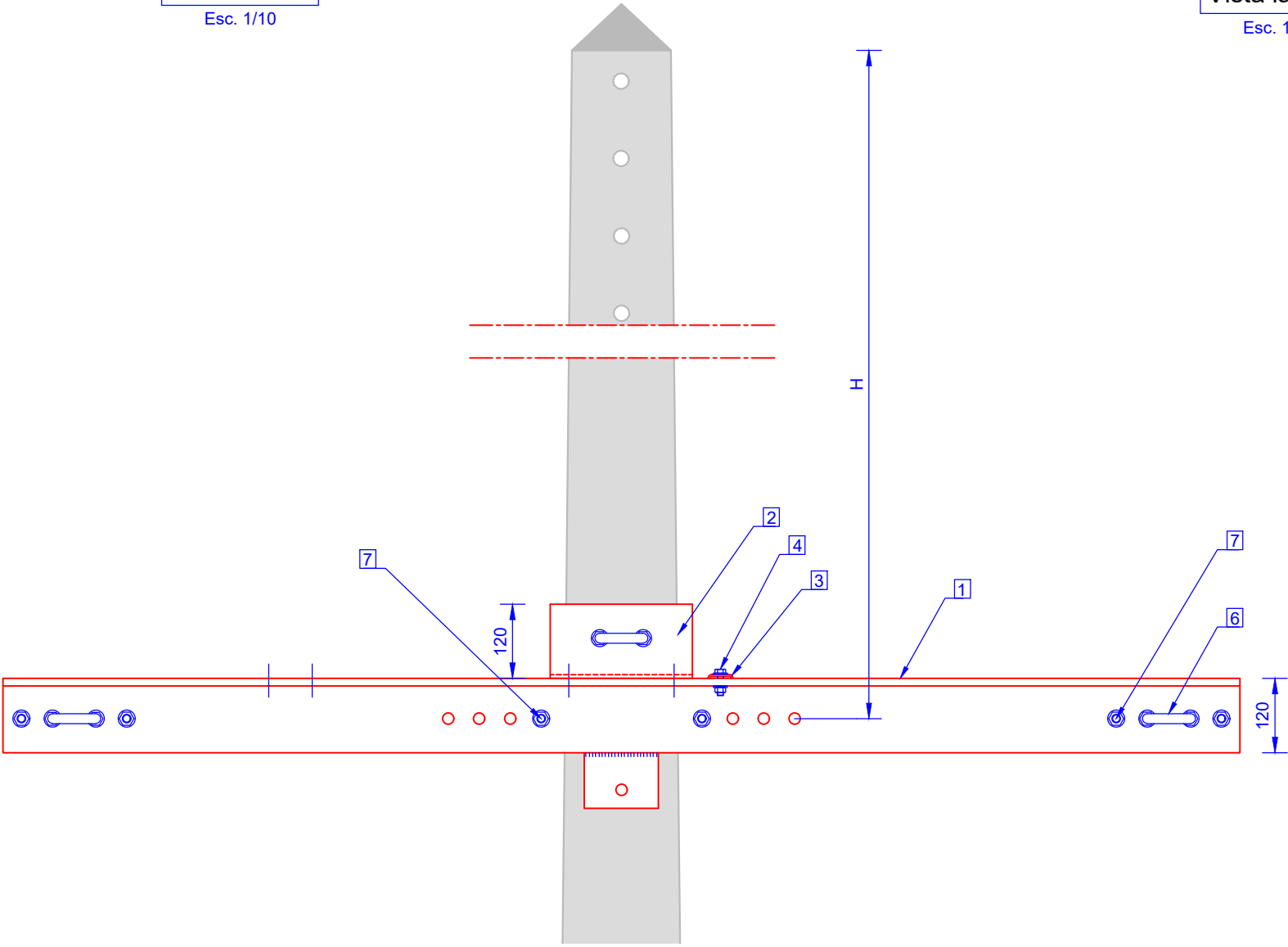
Vista frontal
