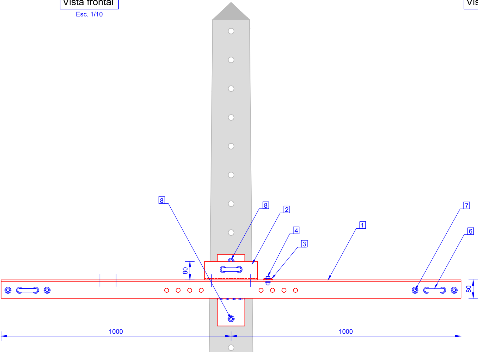
Vista frontal
