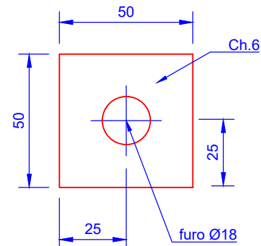
4 AQ50x6 (Esc 1/2)
