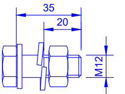
4 M12x35x20+P(1)+AP(1)+AM(1) (Esc 1/2)
