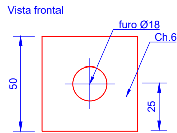
7 AQ50x6 (Esc 1/2)
