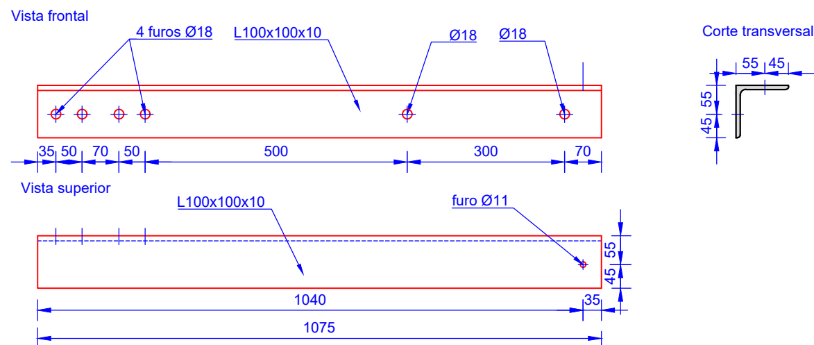
1e L100x100x10 (Esc 1/10)
