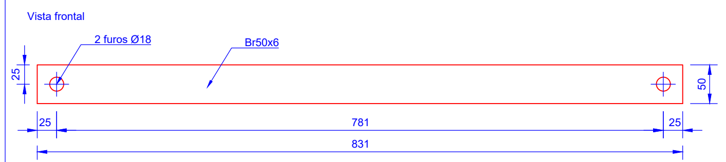
2 Br50x6 (Esc 1/5)
