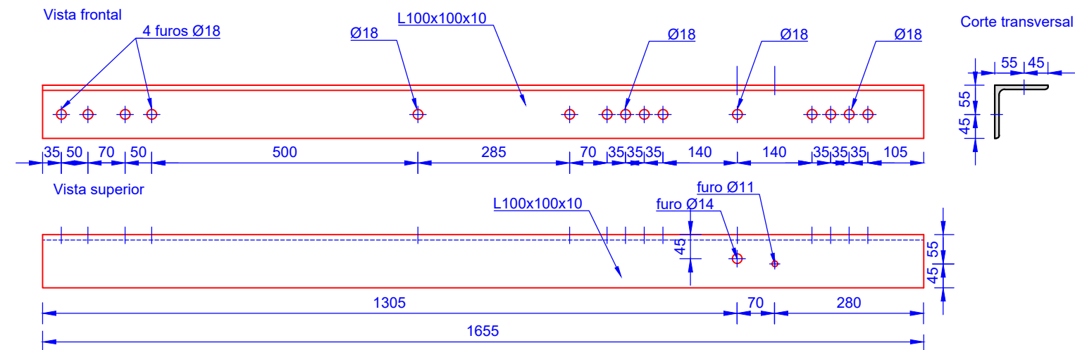
1e L100x100x10 (Esc 1/10)
