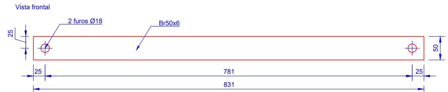
4 Br50x6 (Esc 1/5)
