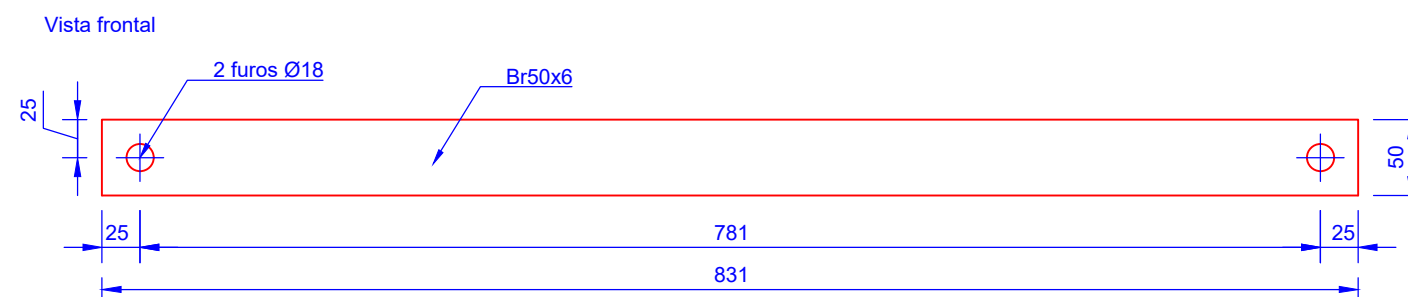
4 Br50x6 (Esc 1/5)
