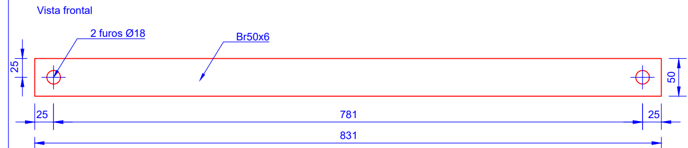
2 Br50x6 (Esc 1/5)
