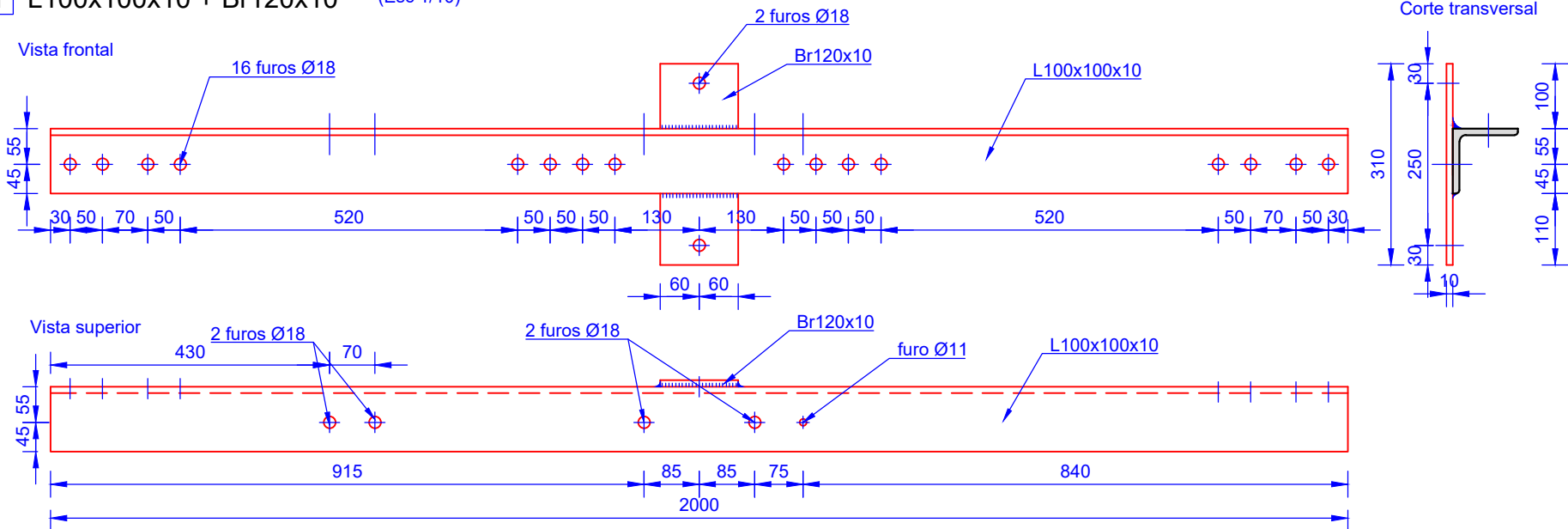
1 L100x100x10 + Br120x10 (Esc 1/10)
