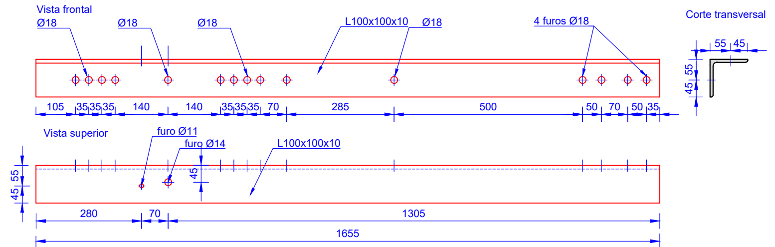
2e L100x100x10 (Esc 1/10)
