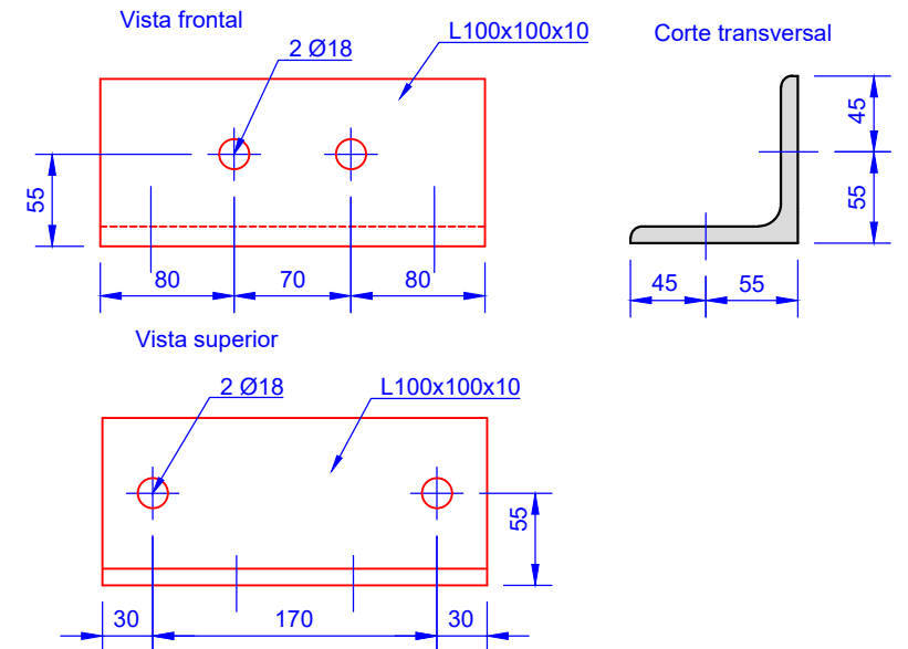
2 L100x100x10 (Esc 1/5)
