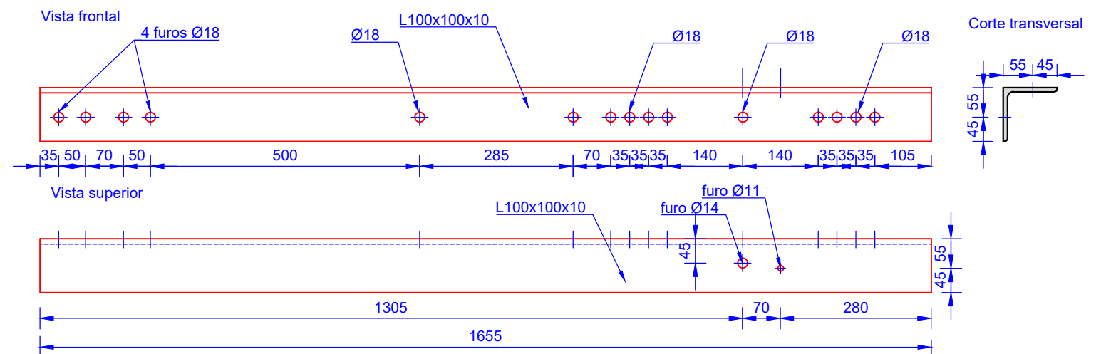
2e L100x100x10 (Esc 1/10)
