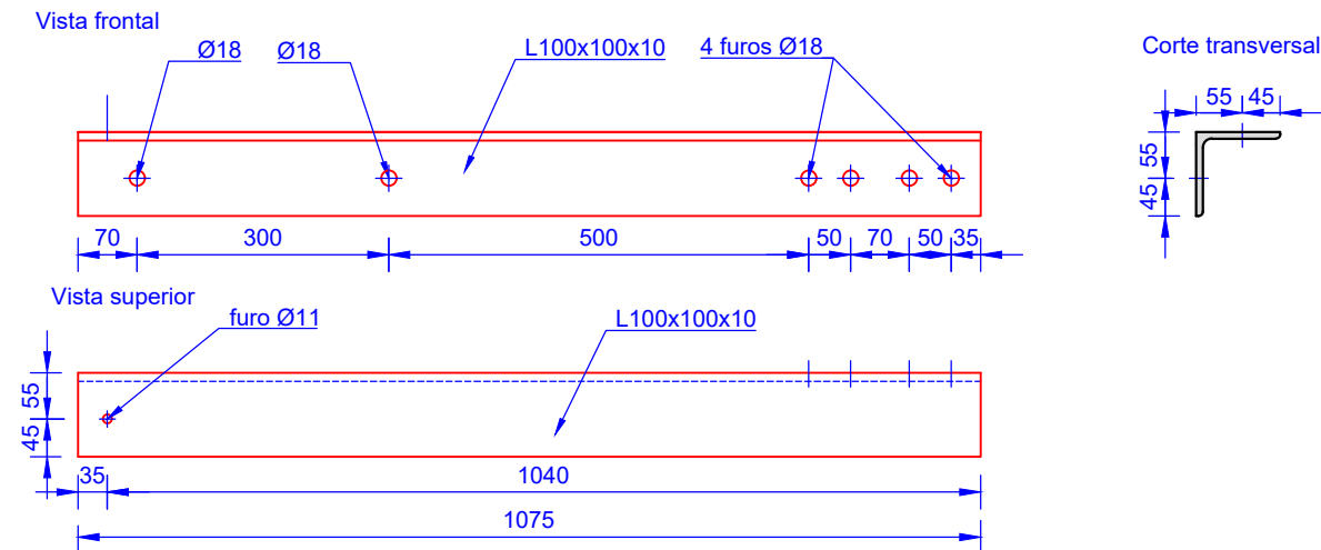
1e L100x100x10 (Esc 1/10)
