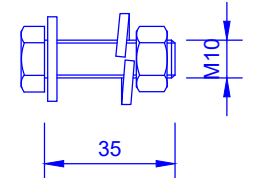
4 M10x35+P(1)+AP(1)+AM(1) (Esc 1/2)
