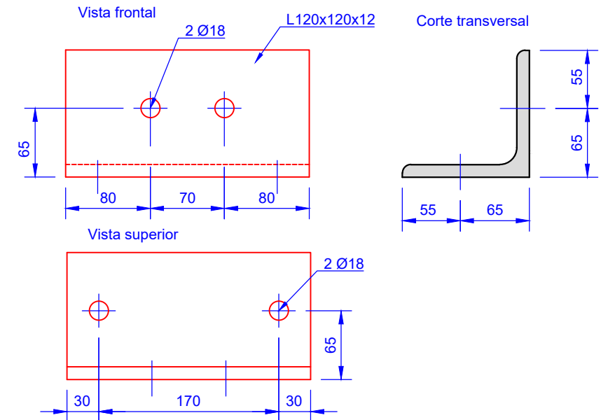
2 L120x120x12 (Esc 1/5)
