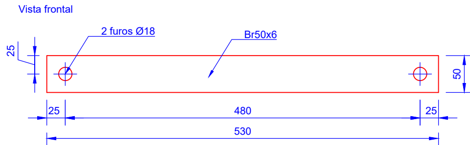
2 Br50x6 (Esc 1/10)
