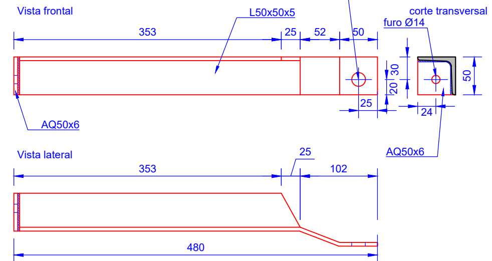
3 L50x50x5 + AQ50x6 (Esc 1/5)
