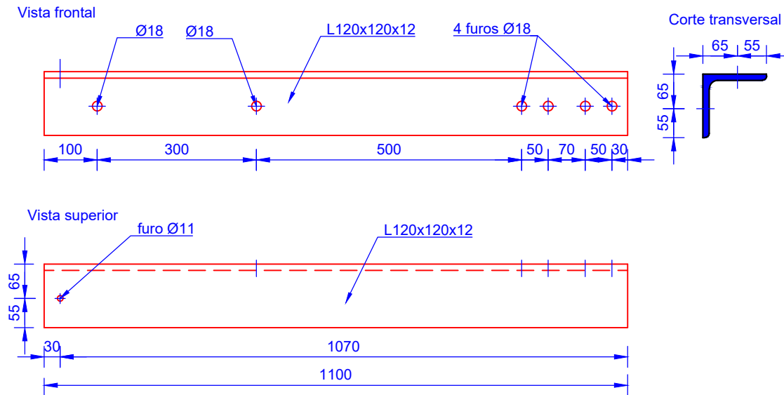
1d L120x120x12 (Esc 1/10)
