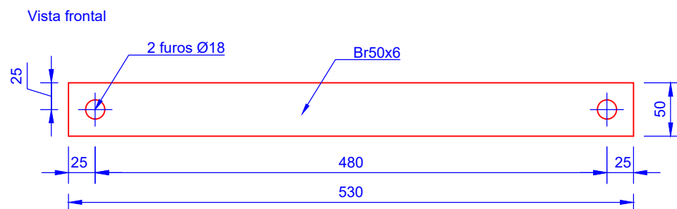
3 Br50x6 (Esc 1/5)
